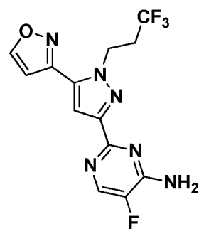
I-513
