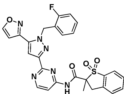
I-594
