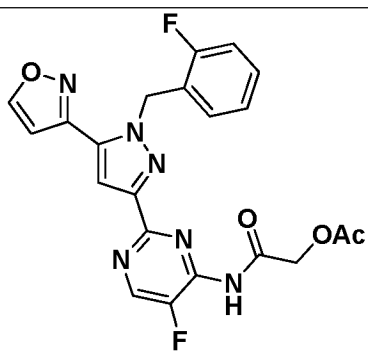
I-498
