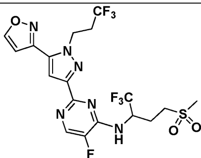
I-626
