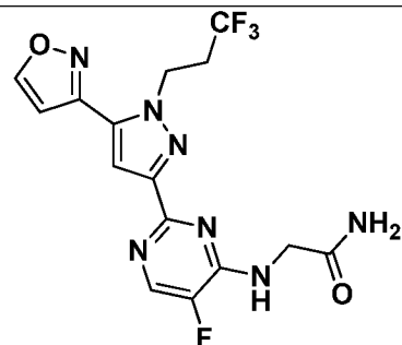
I-511
