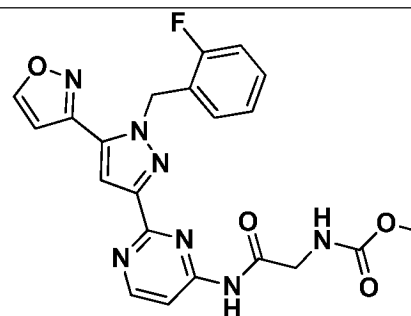
I-603
