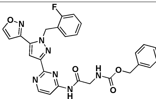
I-598
