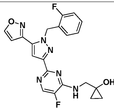
I-359
