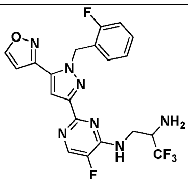
I-518
