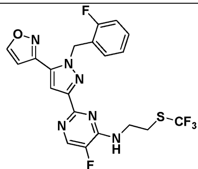
I-509
