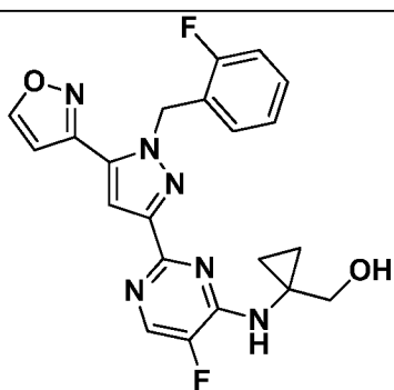
I-502
