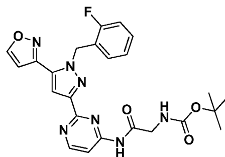
I-519
