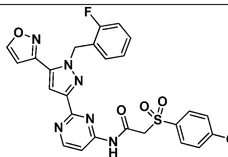
I-593
