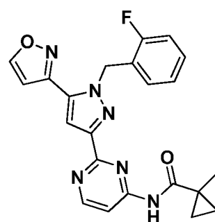
I-569
