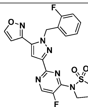
I-503
