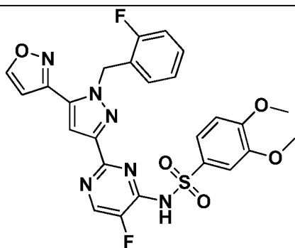
I-614
