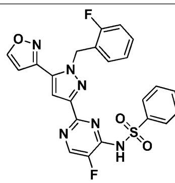
I-613
