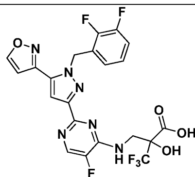
I-489
