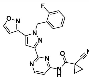
I-551
