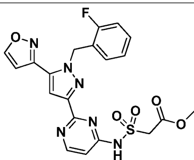
I-510
