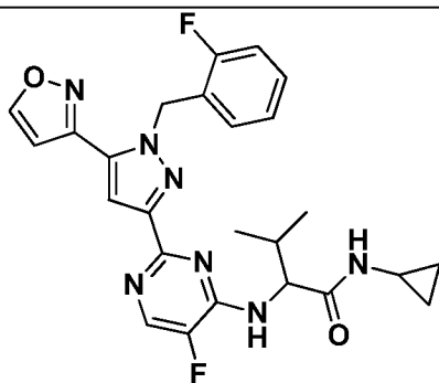
I-508
