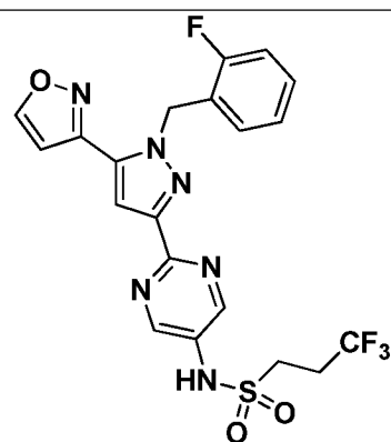
I-595
