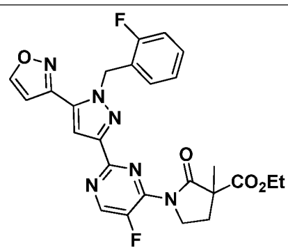
I-591
