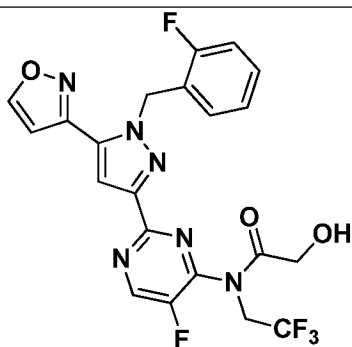
I-566
