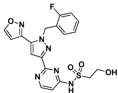
I-539
