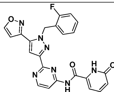
I-553
