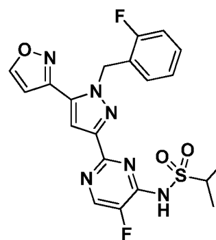
I-505
