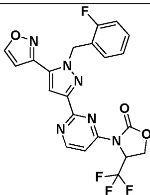
I-504
