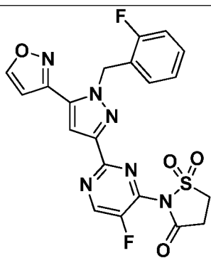
I-612
