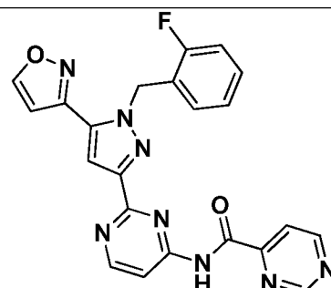
I-553
