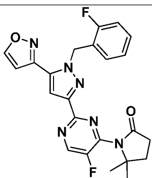
I-512
