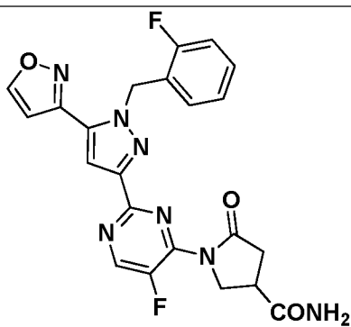
I-590
