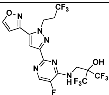
I-516
