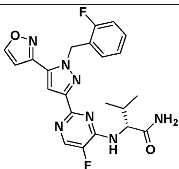
I-536
