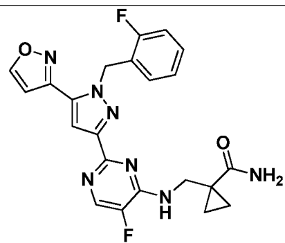
I-515
