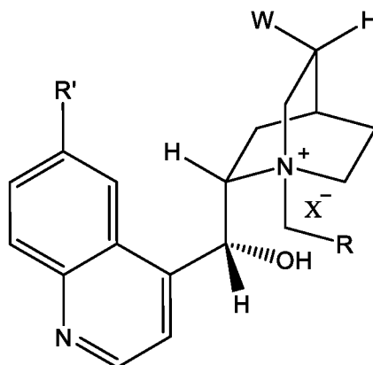
(IIIa)
