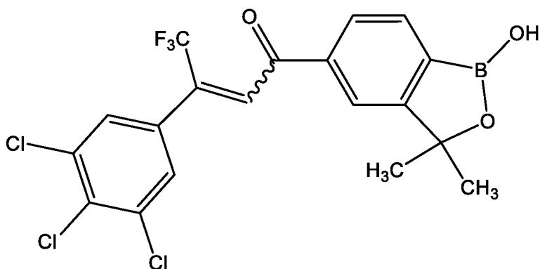
(IIA-1)
