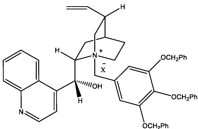
(IIIa-13-3)
