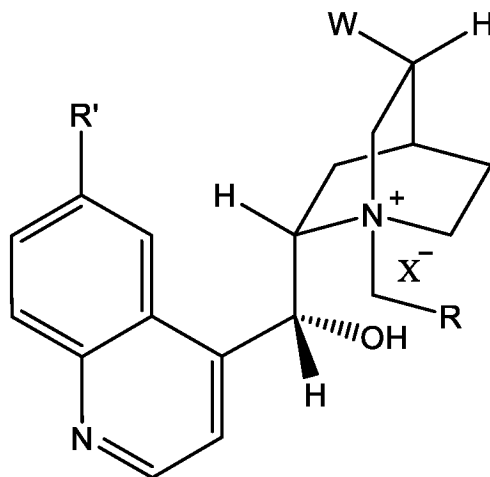
(IIIa)
