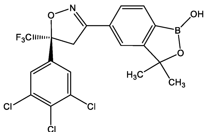
(S)-IE-1
