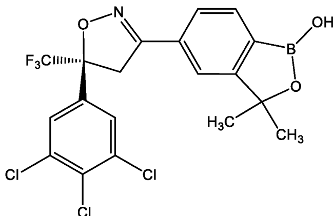
(S)-ID-1
