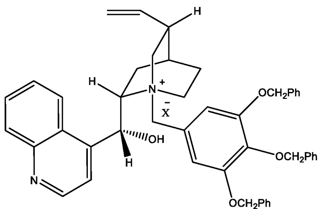
(IIIa-13-3)
