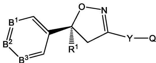
(S)-I
