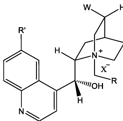
(IIIa)
