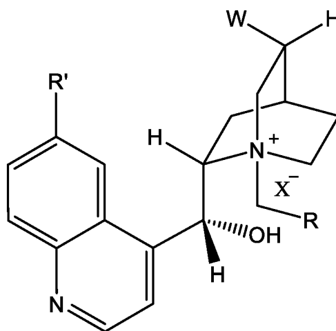
(IIIa)
