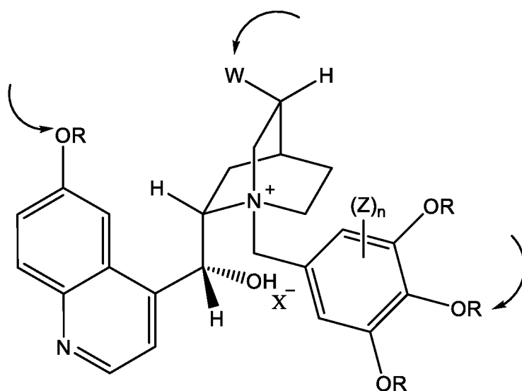
(IIIa-13)
