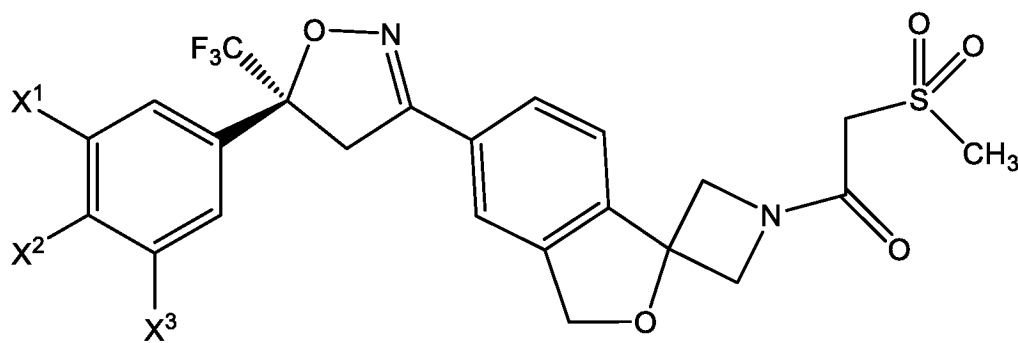
(S)-IC
