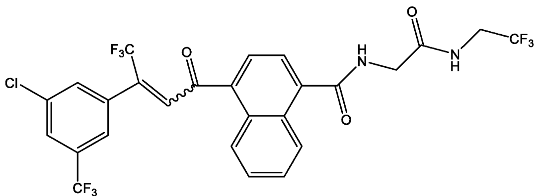
(IIA-1)
