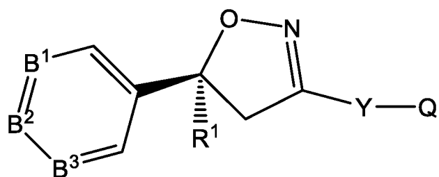
(S)-I
