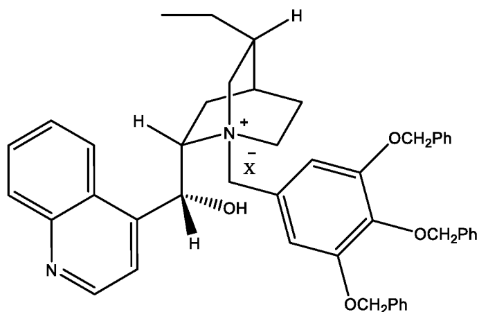
(IIIa-13-4)
