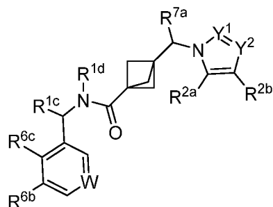
(VIa),
