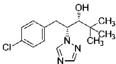
(2R,3R)-
