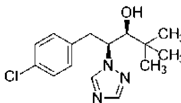
(2S,3S)-
