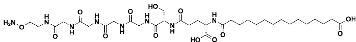
GGGGS-Glu 7 -C14-COOH
